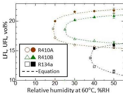
図 2-3 不燃性冷媒 R410A, R410B, R134a の燃焼限界に対する高湿度の影響 Measured at 60°C. Broken curves are fitting functions expressed by Eq. (2-5).
