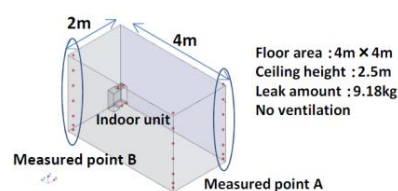
CFD model for floor standing unit
