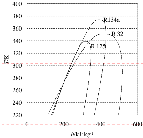
Fig.1 Temperature-enthalpy diagram of R 32, R 125 and R134a.
